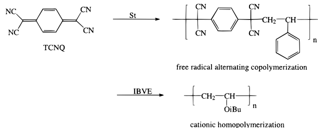
Scheme 5. Polymerization Behavior of TCNQ
